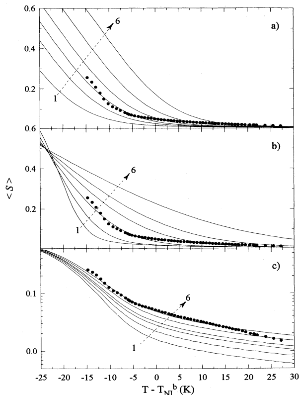
FIG. 7. Six model calculated \langle S \rangle (solid lines) overlaid by the experimental results for 5CB ( \bullet ); (a) 2h_0/a varies in order as 4, 10, 15, 19, 25, and 30 K, respectively, with 2\sigma/a = 10 \text{ K} and g = 1 \times 10^5 \text{ J/m}^3 ; (b) 2\sigma/a varies in order as 3, 6, 10, 15, 20, 30 K, respectively, with 2h_0/a = 22 \text{ K} and g = 1 \times 10^5 \text{ J/m}^3 ; and (c) g varies in order as 7, 8, 9, 10, 11, 12 \times 10^4 \text{ J/m}^3 , respectively, with 2h_0/a = 22 \text{ K} and 2\sigma/a = 4 \text{ K} .
