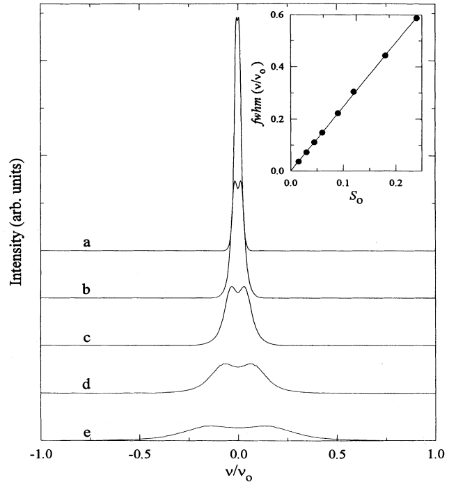
FIG. 6. DNMR line shape simulation based on a superposition of spherical powder patterns having a Gaussian distribution in the scalar order parameter S . The simulations labeled a-e have S_0 (a scaling factor shifting the center of the distribution) progressively doubled. Inset: the normalized FWHM of the simulated line shape versus S_0 showing its linear behavior.
