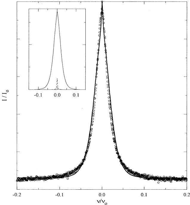
FIG. 9. Comparison of a normalized intensity and frequency spectra of 5CB in Vycor ( \circ ) at 29.98 °C to the independent-pore model with the addition of a narrow Lorentzian (solid line). For clarity, only every other data point is plotted. Inset: the separate contributions of the original model (solid line) and narrow Lorentzian (dashed line), the original model accounts for 98% of the total spectra.
