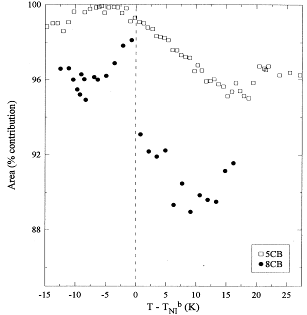
FIG. 4. Percent contribution to the total DNMR peak area of the broad component [ A_B (in %)] which is proportional to the number of orientationally ordered molecules. Note the jump in contribution at T_{NI} for 8CB not seen in 5CB.
