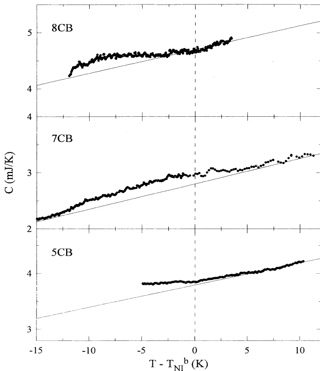
FIG. 5. Heat capacity of 5CB, 7CB, and 8CB (after subtracting the Vycor glass contribution) plotting against T - T_{NI}^b . The highest temperature heat capacity exhibits the same temperature dependence for all liquid crystals. A broad and suppressed “bump” is clearly seen when this high temperature behavior (indicated by the solid line) is extrapolated to lower temperatures.
