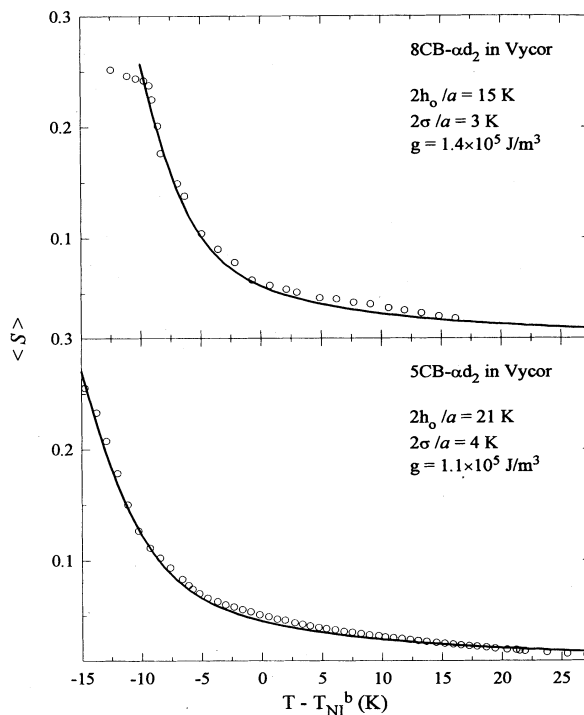
FIG. 8. Best fit to \langle S \rangle for 8CB (top) using 2h_0/a = 15 \text{ K} , 2\sigma/a = 3 \text{ K} , and g = 1.4 \times 10^5 \text{ J/m}^3 , and of 5CB (bottom) using 2h_0/a = 21 \text{ K} , 2\sigma/a = 4 \text{ K} , and g = 1.1 \times 10^5 \text{ J/m}^3 . Using the appropriate Landau expansion coefficient a for each liquid crystal, a consistent mean pore radius of R = 35 \pm 0.5 \text{ \AA} and width of the pore size distribution of 7 \pm 0.5 \text{ \AA} , nearly identical to that determined experimentally by nitrogen isotherms [26] are found.
