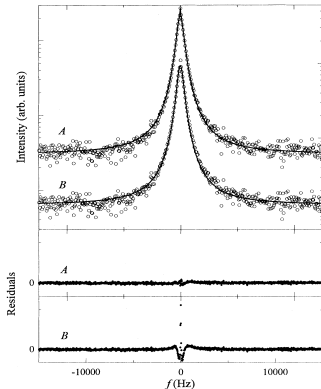
FIG. 2. Semilogarithmic plot of the DNMR absorption spectra for 5CB- \alpha d_2 in Vycor at 55^\circ\text{C} . Fitting with a double Lorentzian (A) yields a near perfect fit compared with a single Lorentzian that fails to fit the data near the peak maximum (B). For clarity, only every other data point is plotted. The residuals of the fits are given in the lower panels with a scale 4% of the upper intensity plot.
