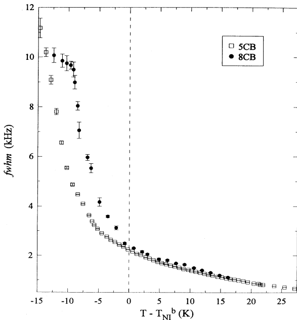
FIG. 3. The FWHM of the broad (orientationally ordered) component for 5CB ( \square ) and 8CB ( \bullet ) confined to Vycor.
